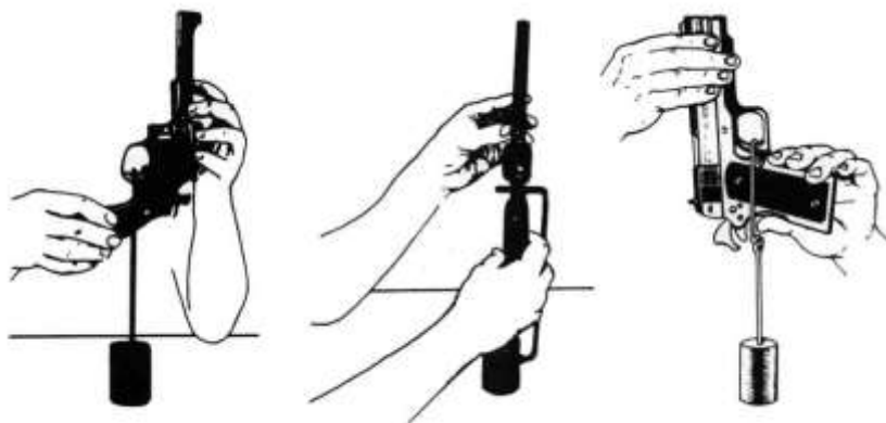
CORRECT METHOD OF WEIGHING TRIGGERS
